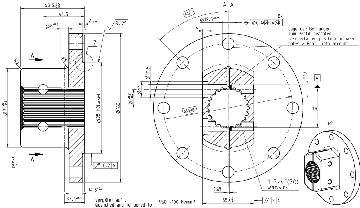
PTO bush 20 teeth (1 3/4"), ≤ 5.000 Nm maximum dynamic constant load
