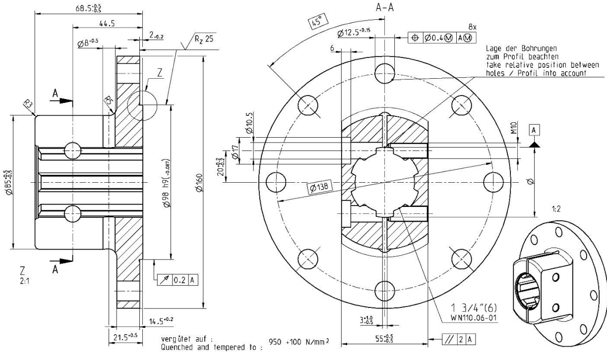
PTO bush 6 teeth (1 3/4"), ≤ 5.000 Nm maximum dynamic constant load
