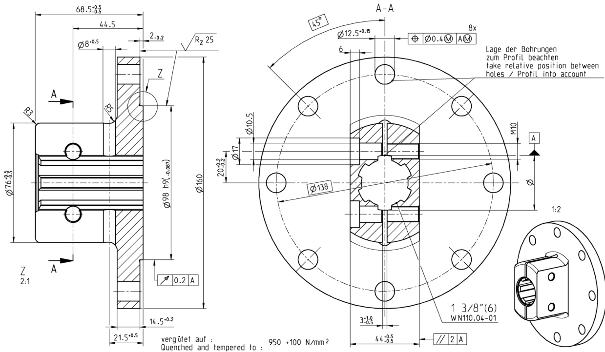
PTO bush 6 teeth (1 3/8"), ≤ 5.000 Nm maximum dynamic constant load
