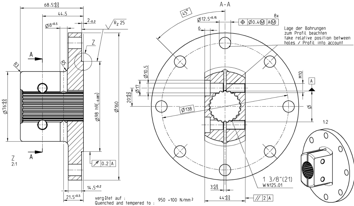
PTO bush 21 teeth (1 3/8"), ≤ 5.000 Nm maximum dynamic constant load
