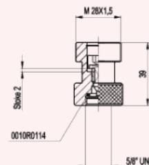
M28x1.5 master valve adaptors
