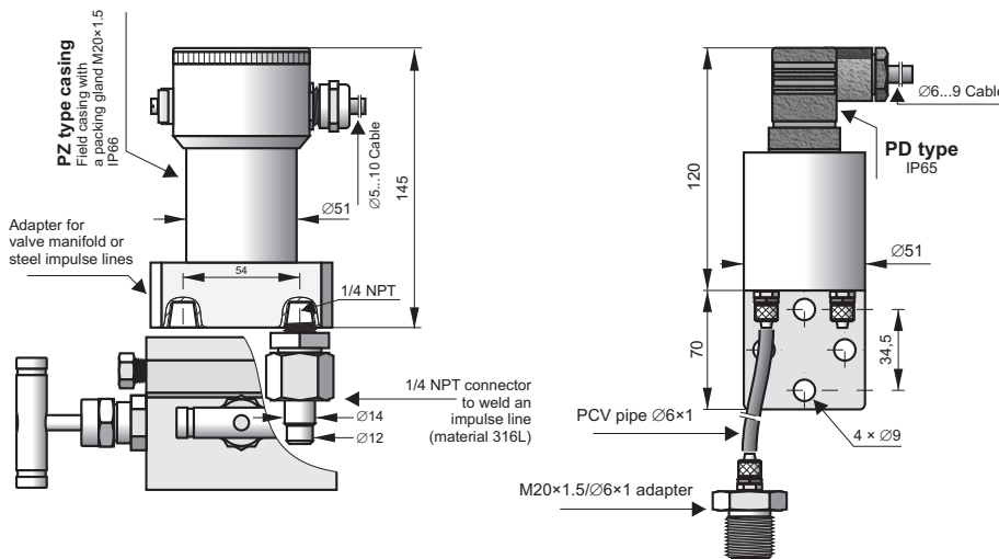
HDPM-2I Industrial Version, C type process connector to be mounted along with a valve manifold an example with PZ type Electrical Connection
